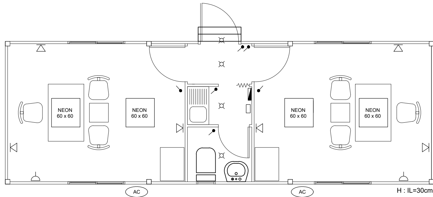
ELECTRICAL LAYOUT
